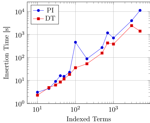
Figure 4.9: Insertion Performance
