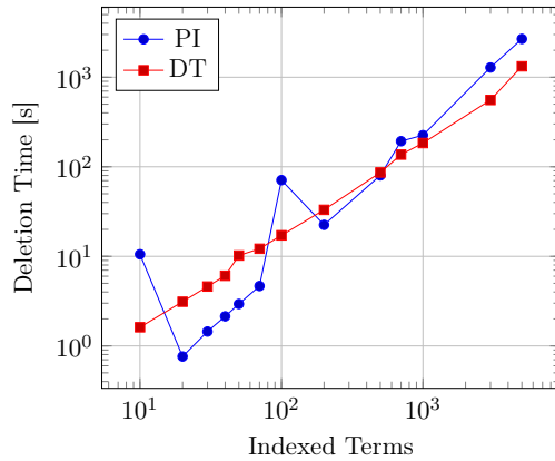
Figure 4.10: Deletion Performance
